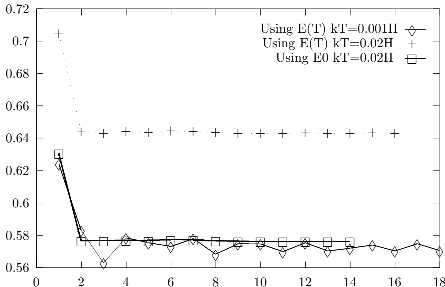
Figure 2.5: The surface energy (J/M 2 ) of Li(100) for various numbers of layers in a slab model showing the effects of WIDTH (0.02H and 0.001H) and the use of E(T) or E0
